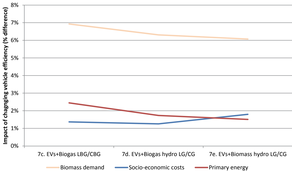
Figure 35: Impacts of reducing the gas vehicle efficiencies on biomass demand, socio-economic costs and primary energy demand
